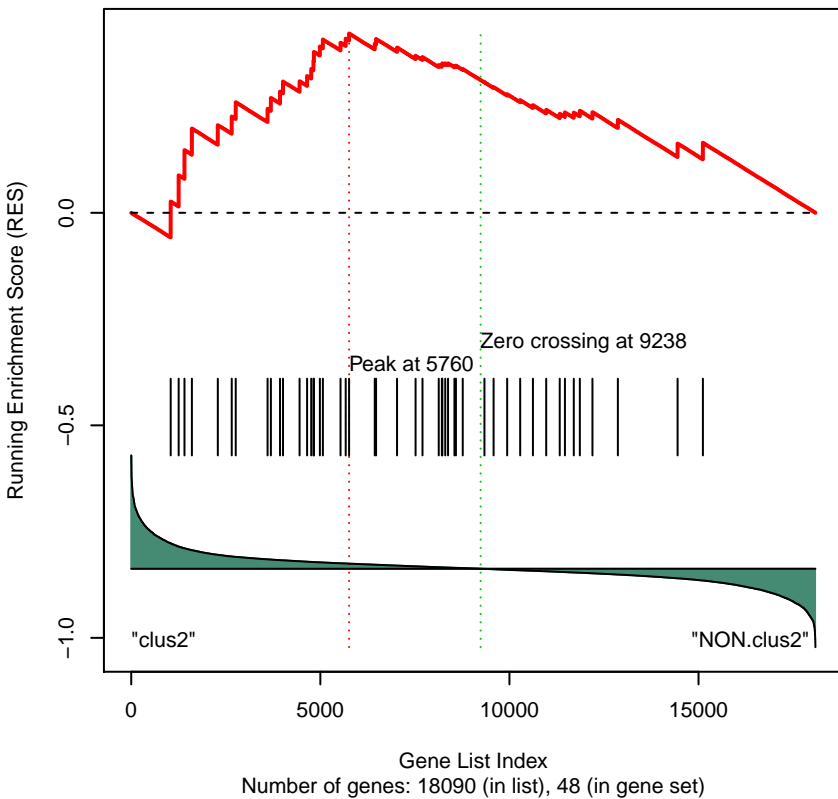
Gene Set 306 : PID_CERAMIDE_PATHWAY
