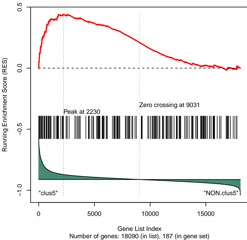
Gene Set 538 : REACTOME_TRANSCRIPTION
