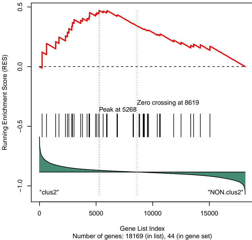
Gene Set 14 : KEGG_LYSINE_DEGRADATION
