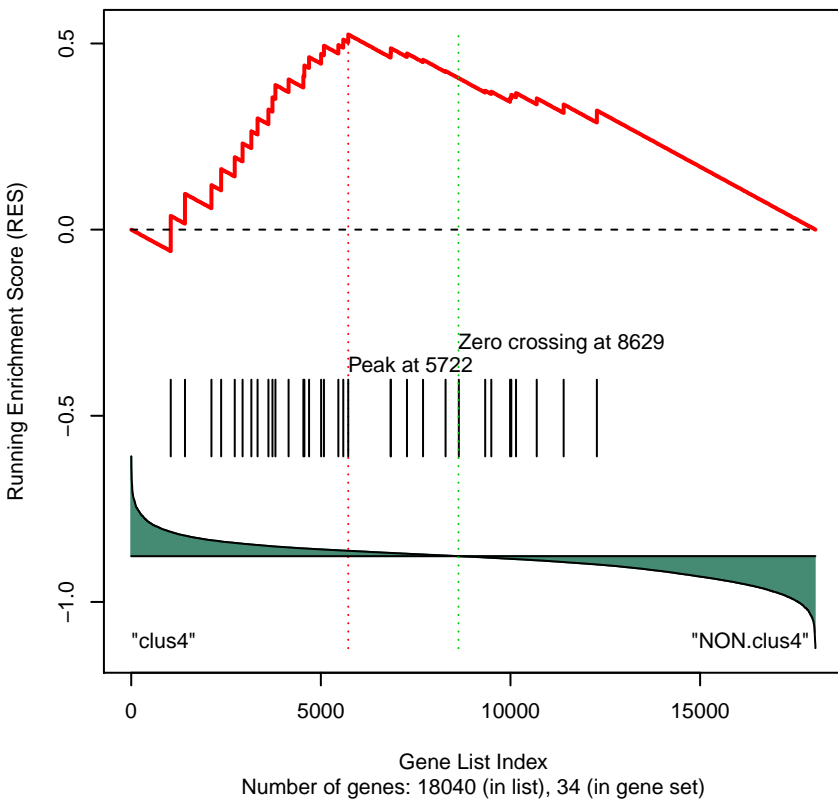
Gene Set 271 : PID_ATM_PATHWAY
