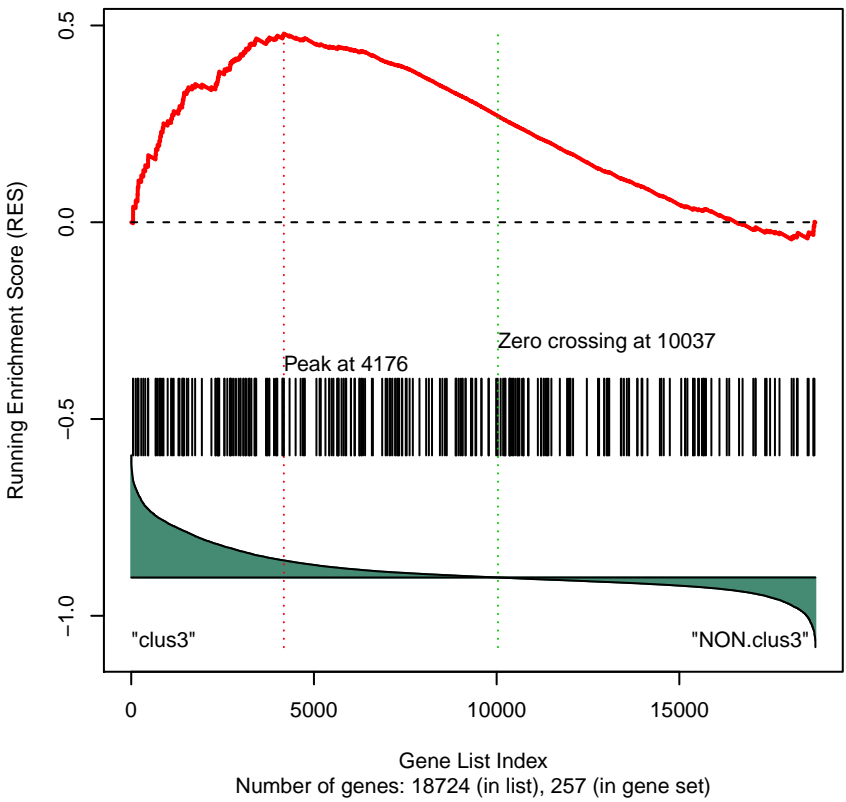
Gene Set 58 : KEGG_MAPK_SIGNALING_PATHWAY
