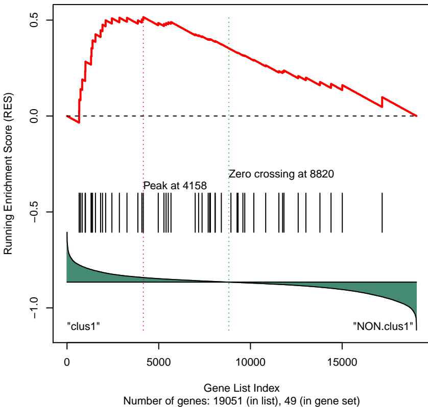
Gene Set 305 : PID_PI3KCIPATHWAY
