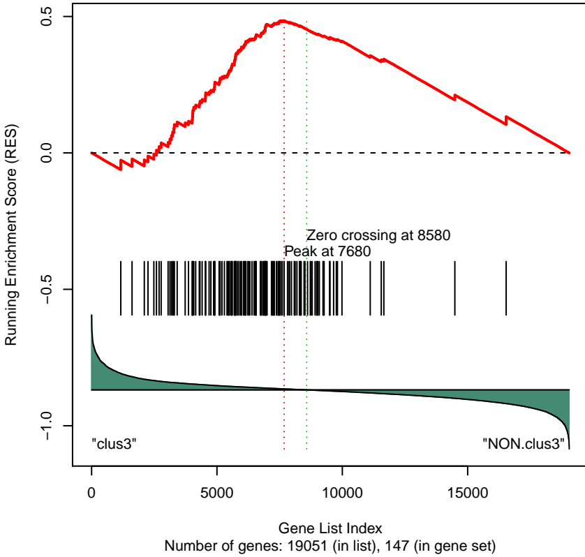
Gene Set 386 : REACTOME_TRANSLATION
