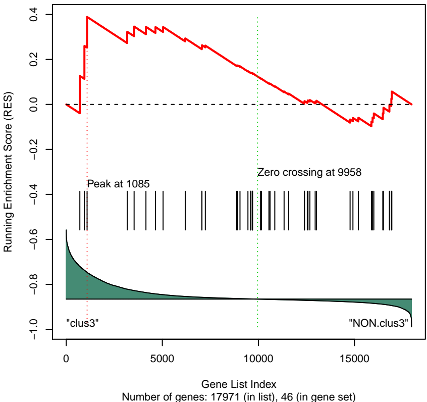
Gene Set 20 : KEGG_GLUTATHIONE_METABOLISM
