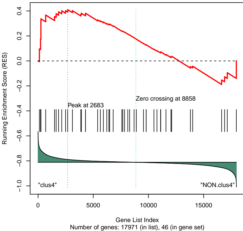
Gene Set 299 : PID_AJDISS_2PATHWAY
