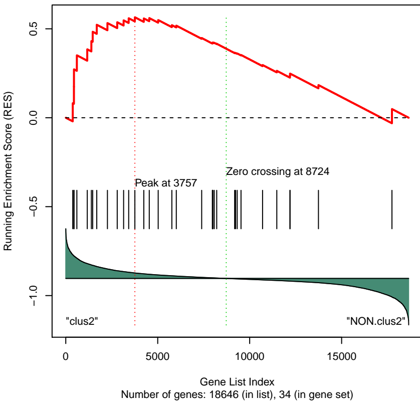
Gene Set 287 : PID_IL1PATHWAY
