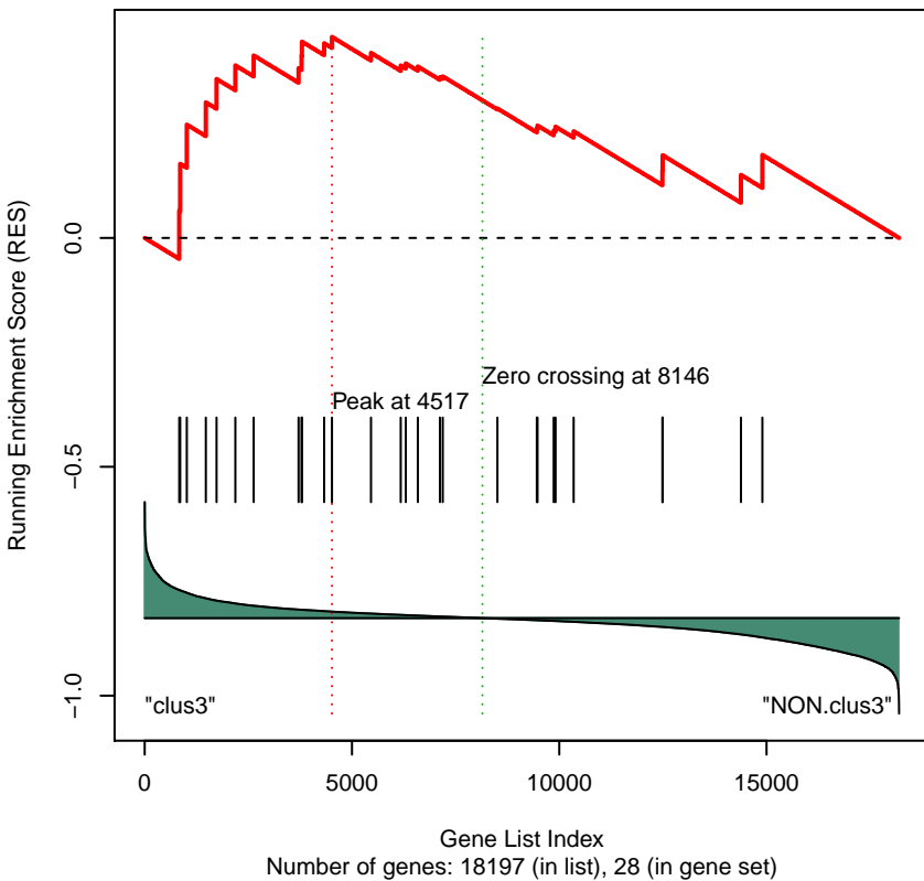
Gene Set 272 : PID_TRAIL_PATHWAY
