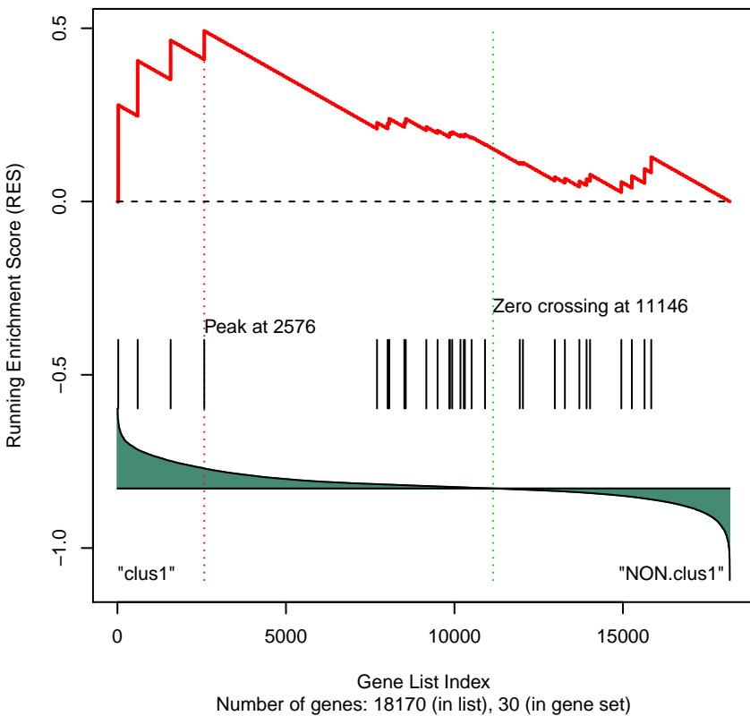
Gene Set 294 : PID_IGF1_PATHWAY
