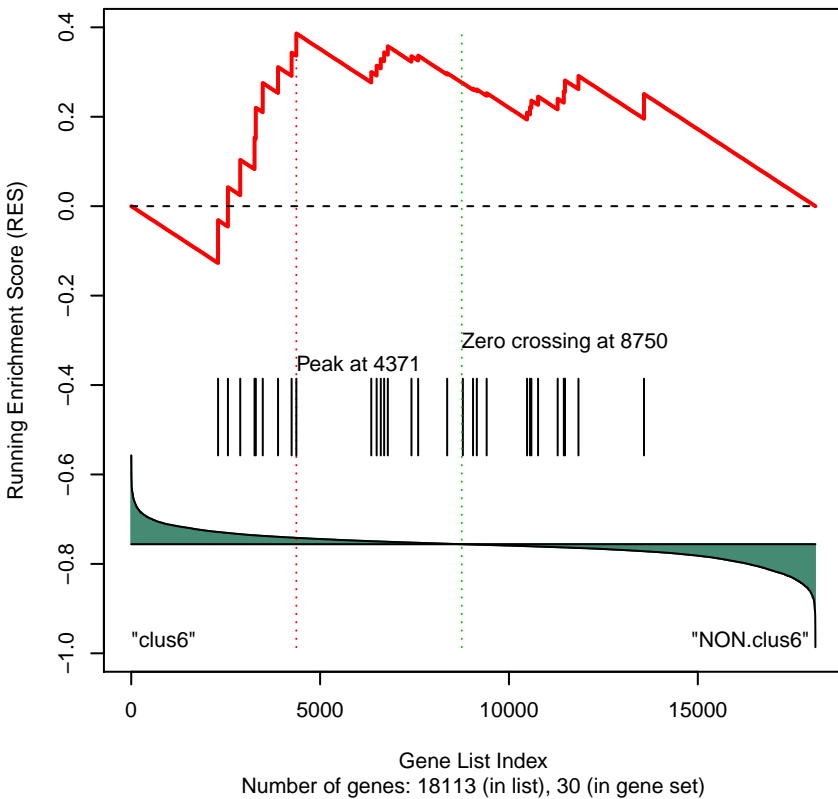
Gene Set 271 : PID_NECTIN_PATHWAY
