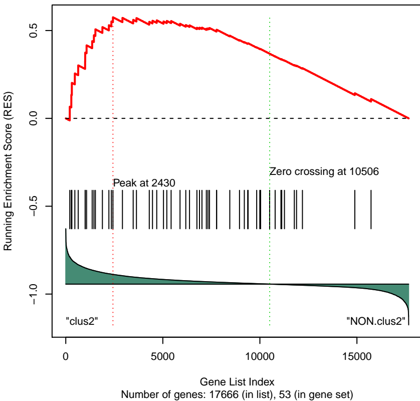
Gene Set 276 : PID_CD8TCRPATHWAY
