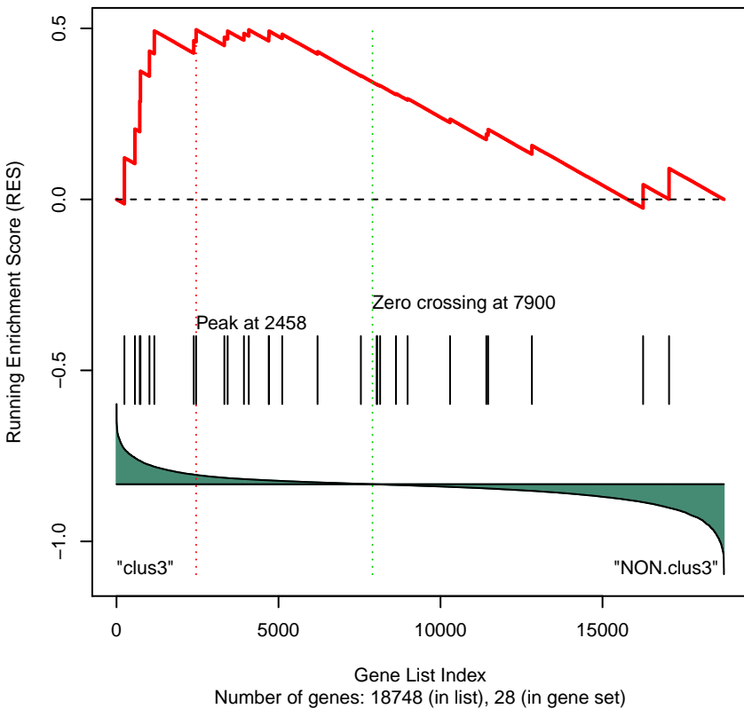
Gene Set 164 : BIOCARTA_ERK_PATHWAY
