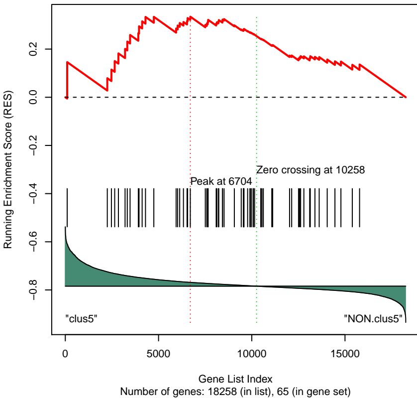
Gene Set 287 : PID_HDAC_CLASSI_PATHWAY
