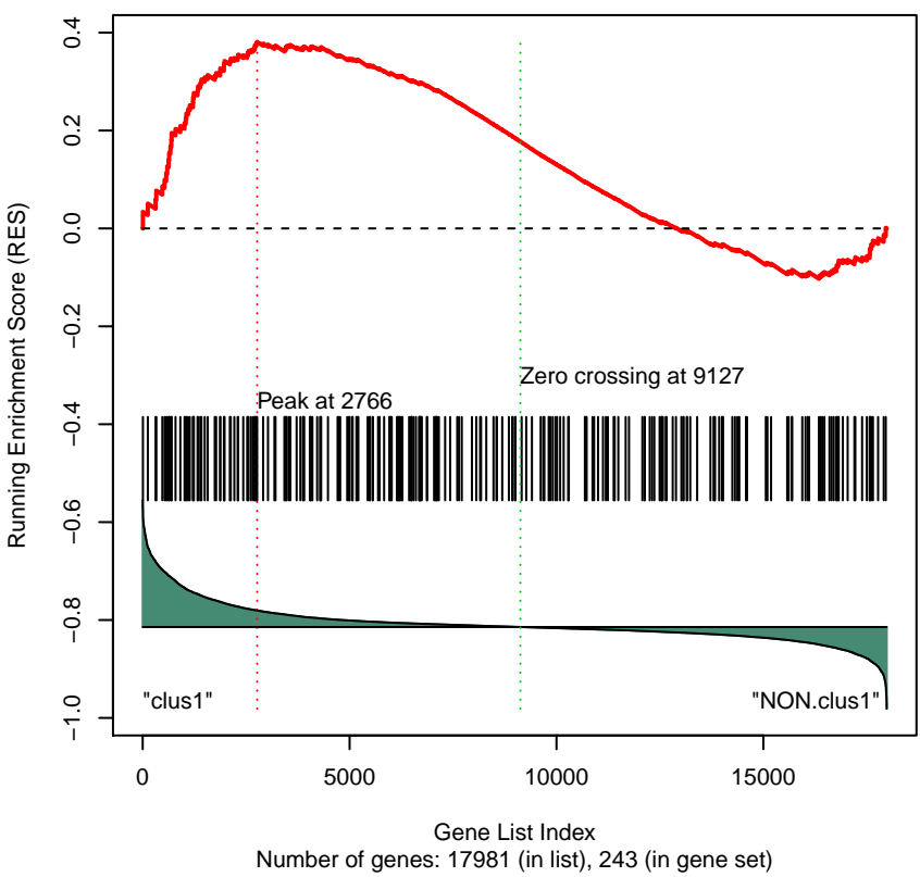
Gene Set 57 : KEGG_MAPK_SIGNALING_PATHWAY
