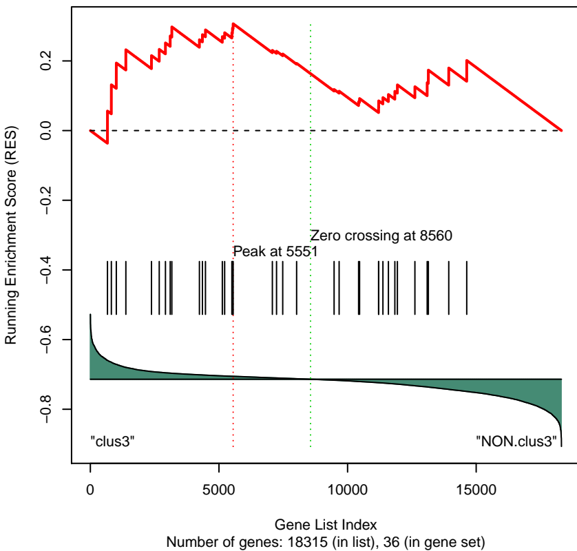
Gene Set 456 : REACTOME_PI3K_AKT_ACTIVATION
