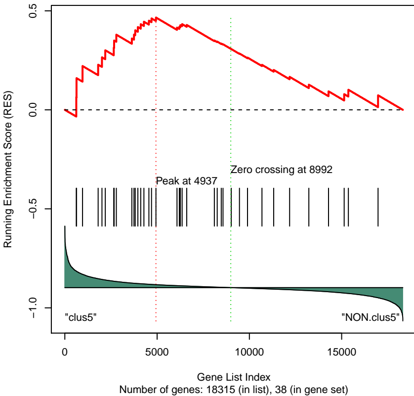
Gene Set 6 : KEGG_FATTY_ACID_METABOLISM
