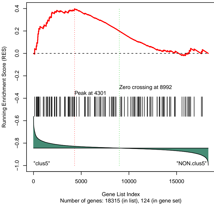
Gene Set 84 : KEGG_TIGHT_JUNCTION
