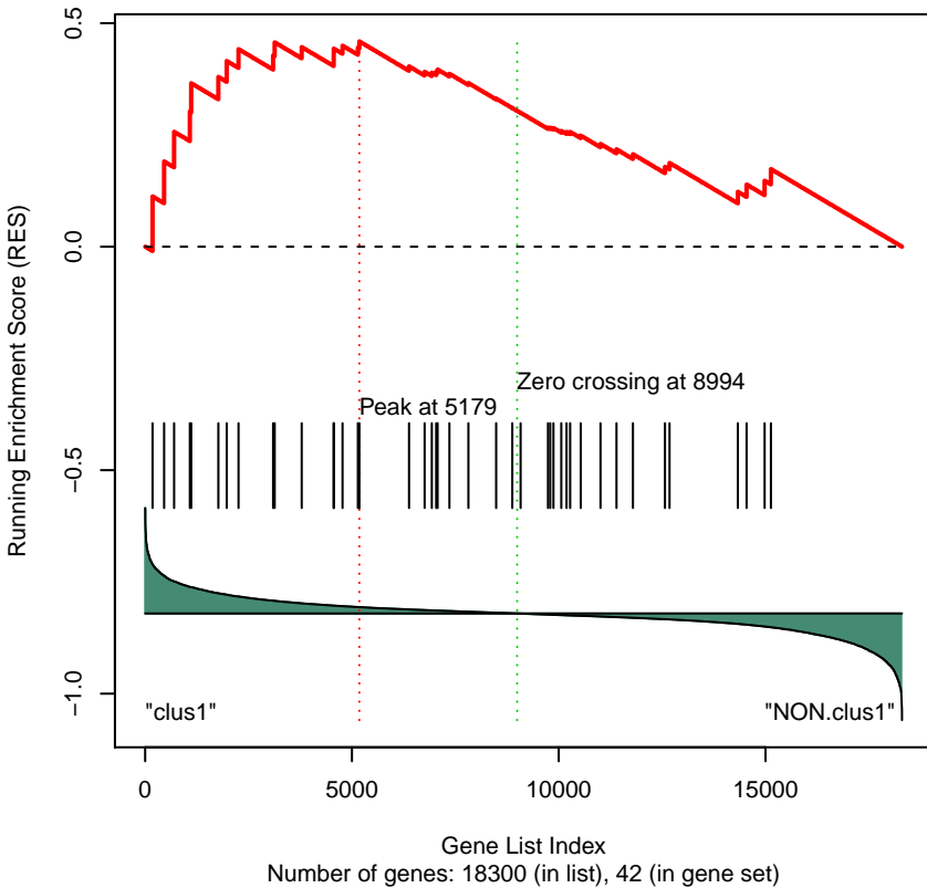
Gene Set 279 : PID_TCPTP_PATHWAY
