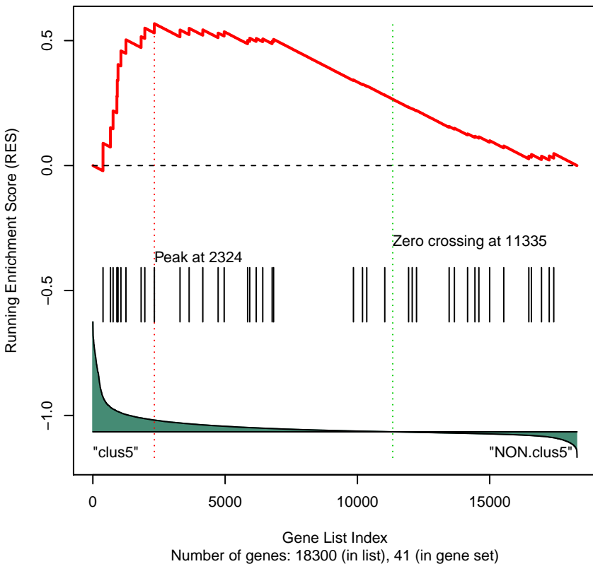
Gene Set 21 : KEGG_STARCH_AND_SUCROSE_METABOLISM
