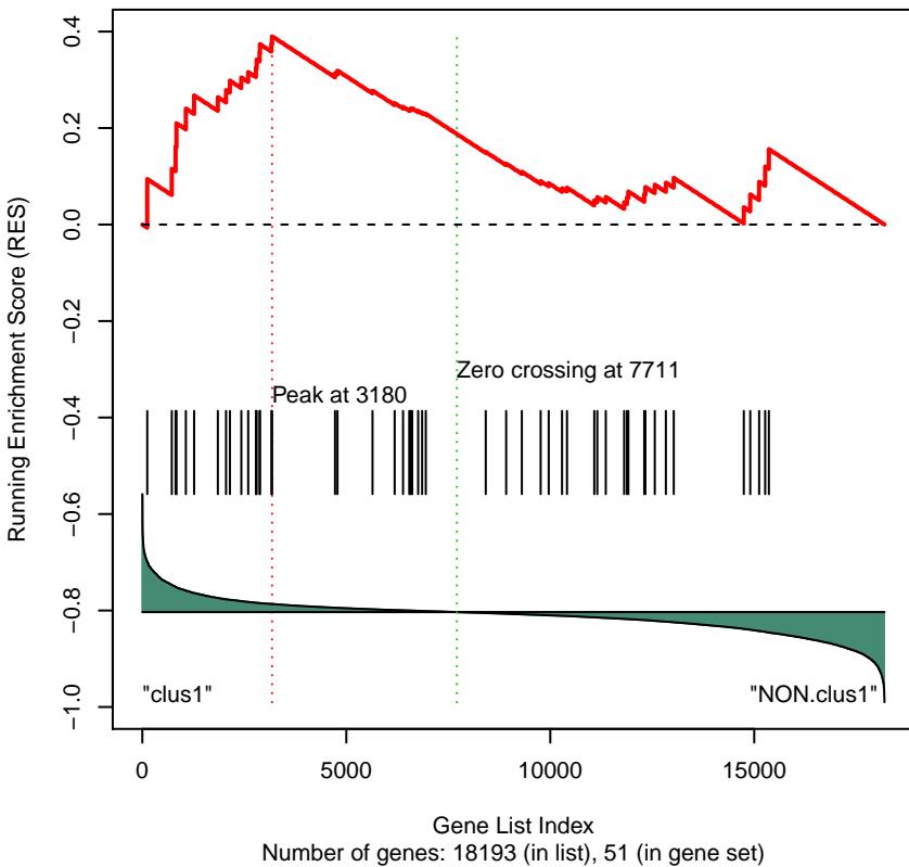
Gene Set 338 : PID_CASPASE_PATHWAY
