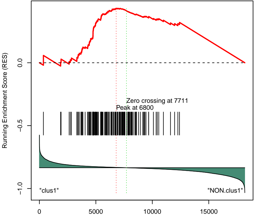
Gene List Index Number of genes: 18193 (in list), 146 (in gene set)
