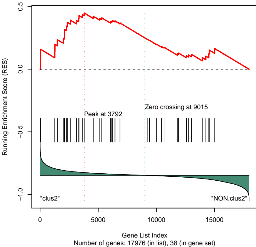
Gene Set 153 : BIOCARTA_BIOPEPTIDES_PATHWAY
