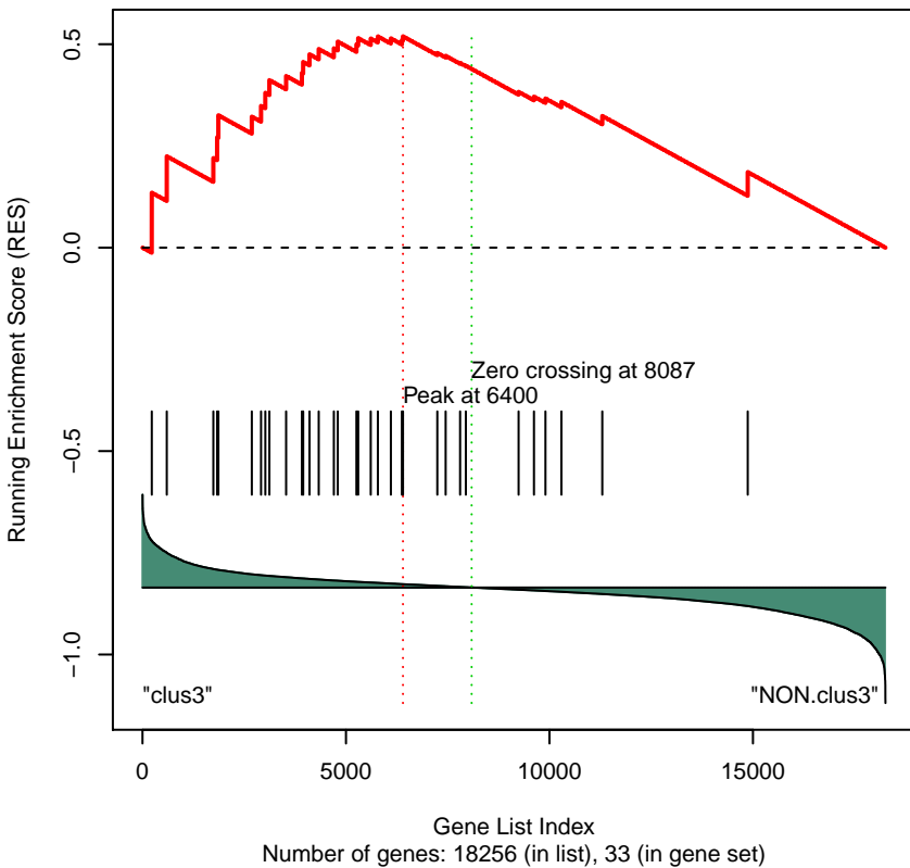
Gene Set 53 : KEGG_BASE_EXCISION_REPAIR
