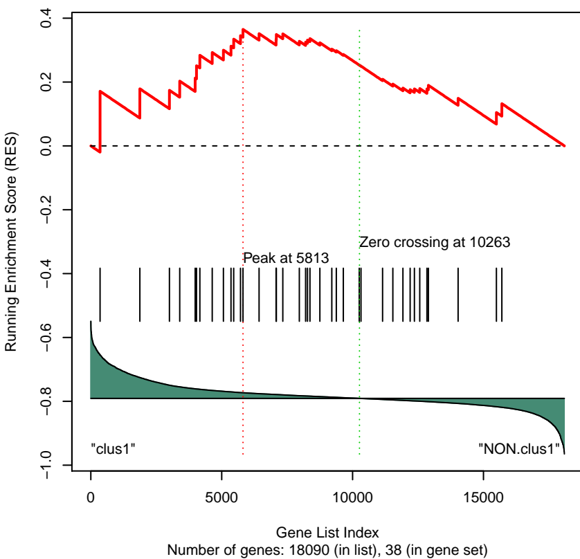
Gene Set 68 : KEGG_SNARE_INTERACTIONS_IN_VESICULAR_TRANSF
