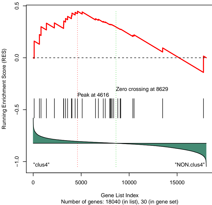
Gene Set 330 : PID_RETINOIC_ACID_PATHWAY
