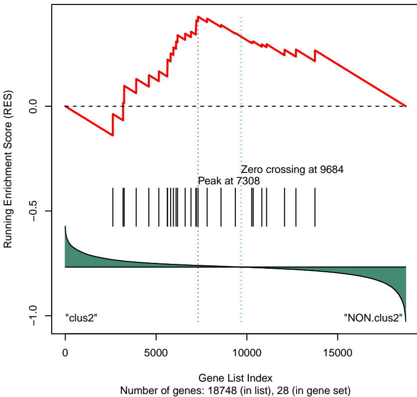
Gene Set 93 : KEGG_RNA_POLYMERASE
