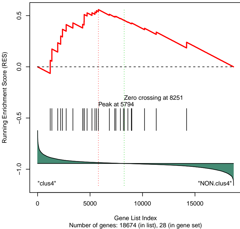
Gene Set 276 : PID_TRAIL_PATHWAY
