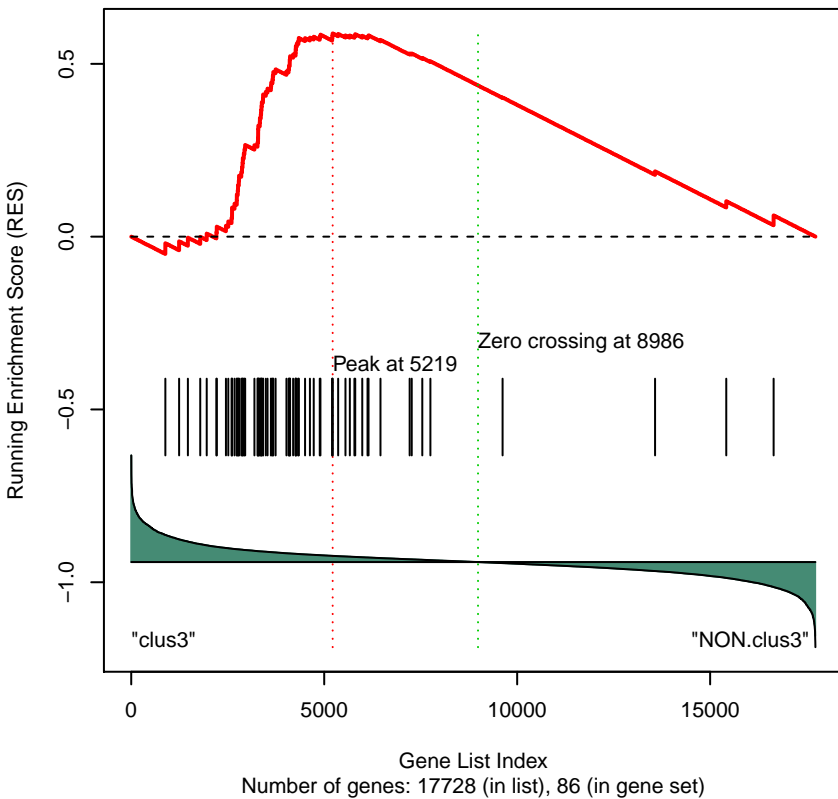
Gene Set 45 : KEGG_RIBOSOME
