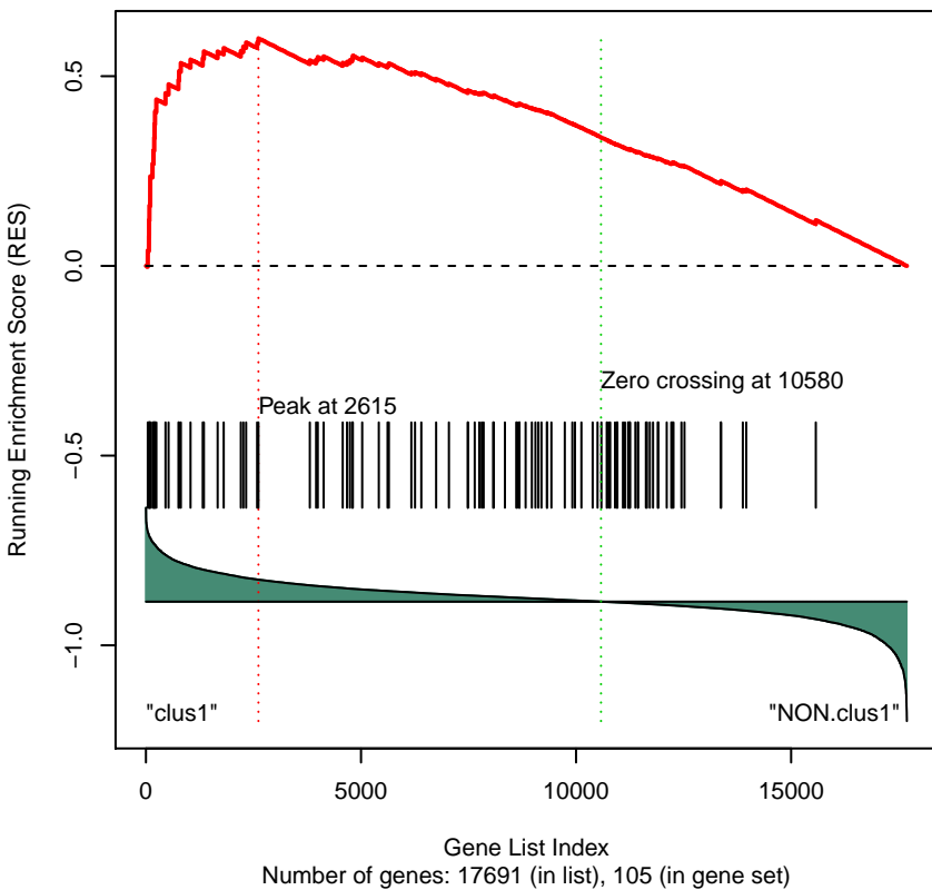
Gene Set 499 : REACTOME_CELL_CYCLE_CHECKPOINTS
