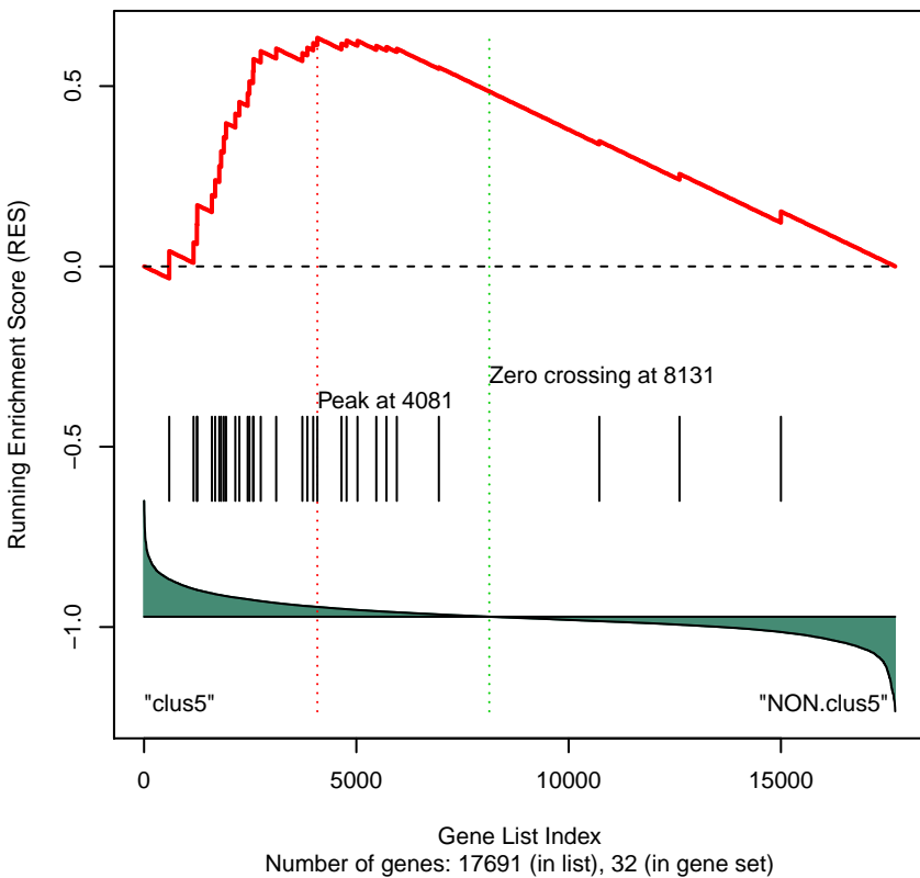
Gene Set 36 : KEGG_PROANOATE_METABOLISM
